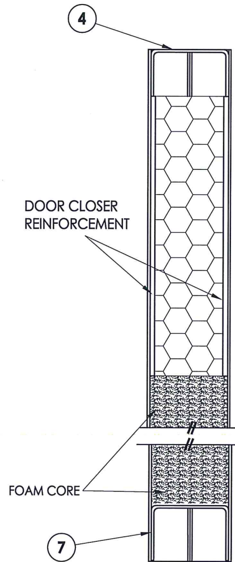
VERTICAL CROSS SECTION
