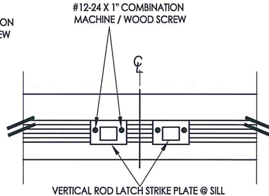
DETAIL 2 Vertical rod latch strike plate @ sill
