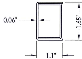
STILE REINFORCEMENT
